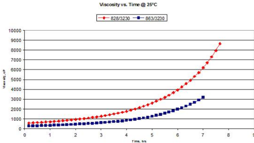
Graph 1 / Viscosity vs. Time at 25°C of EPON Resin 828 & 863 cured with EPIKURE Curing Agent 3230
